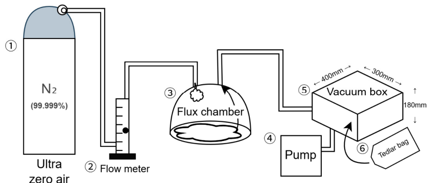
Fig. 2. Flux chamber used in this study. ① High-purity nitrogen, nitrogen with 99.999% purity was used; ② Flow meter (RMA-14-SSV, Dwyer Instruments, Michigan, IN, USA), with a capacity of 200-2,500 cc/min; ③ Flux chamber, which had a volume of 15 L; ④ Pump (VP-18D, Astek, Anyang, Korea); ⑤ Vacuum box (21.6 L, Astek); the pressure-regulating pump and vacuum box were custom-made; ⑥ Tedlar bag (3 L or 5 L, HS Korea).
